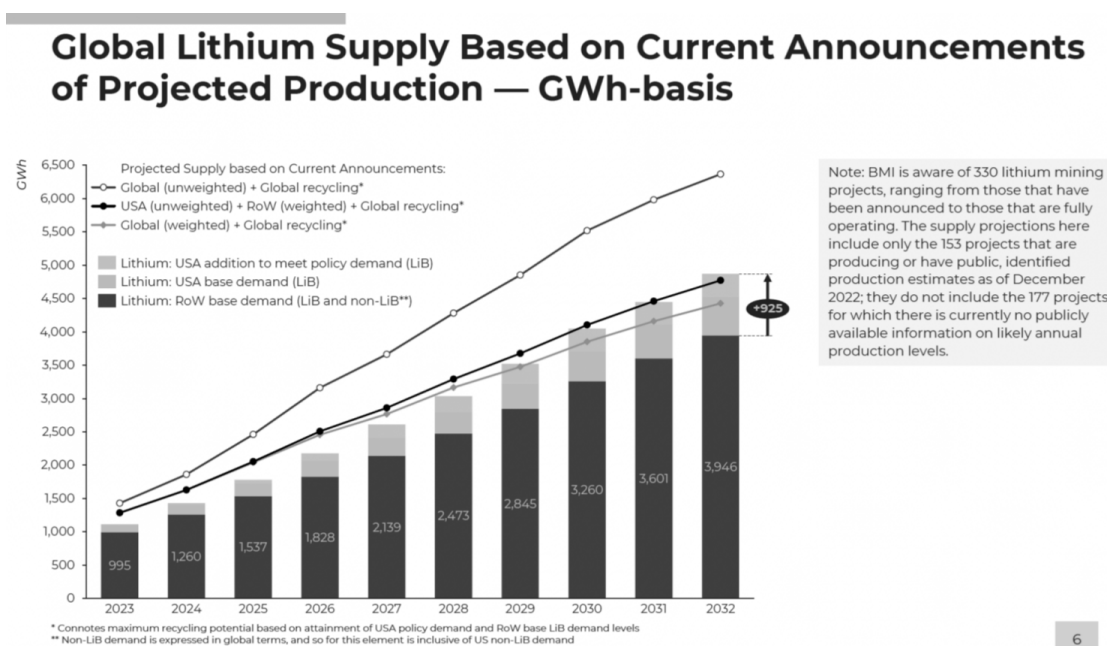
Figure II-3 Global Lithium Supply Based on Current Announcements of Projected Production Along with Global and U.S. Lithium Demand (with demand expressed as GWh)
