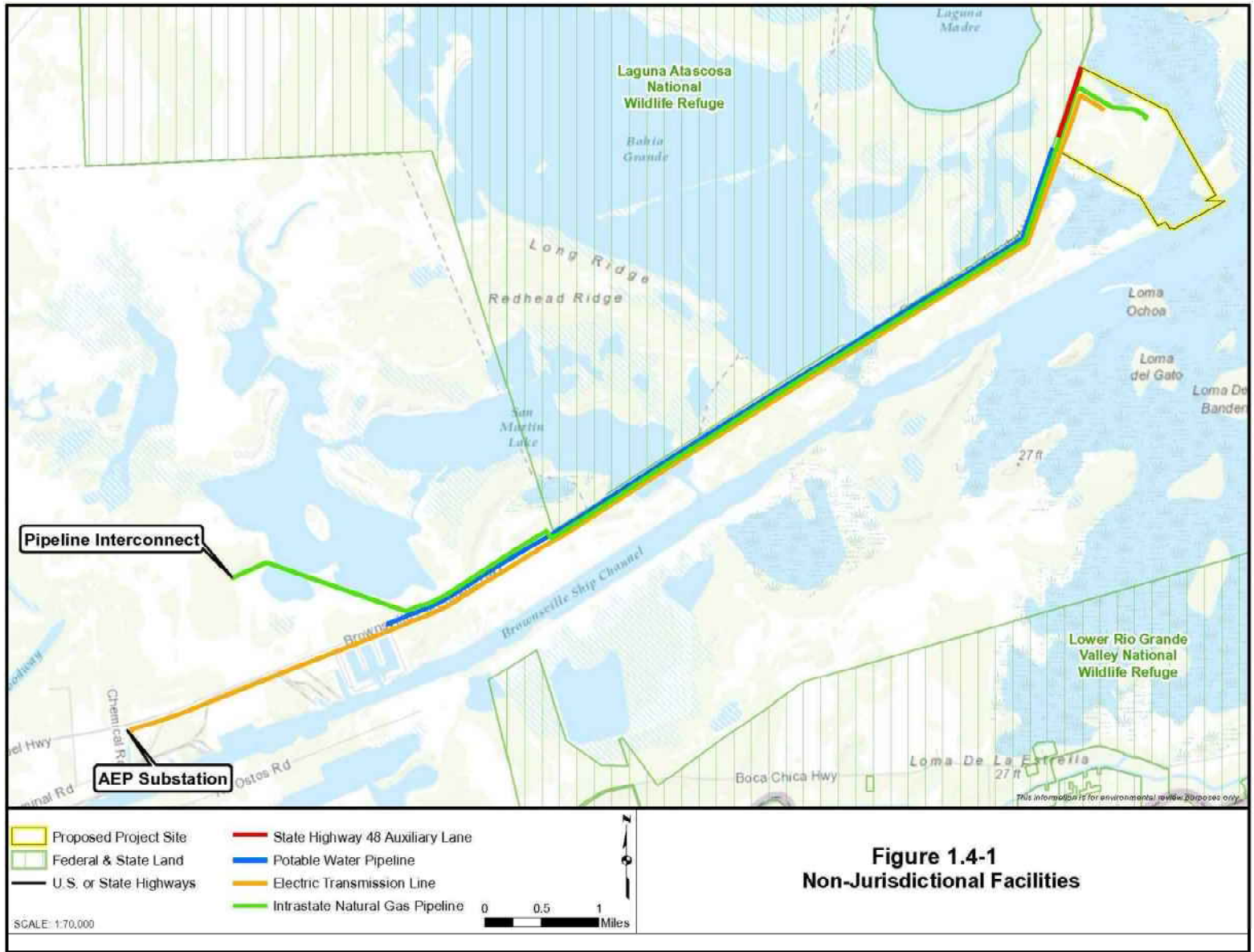
FIGURE 1.4-1 Non-jurisdictional Facilities Associated with the Proposed Texas LNG Project
