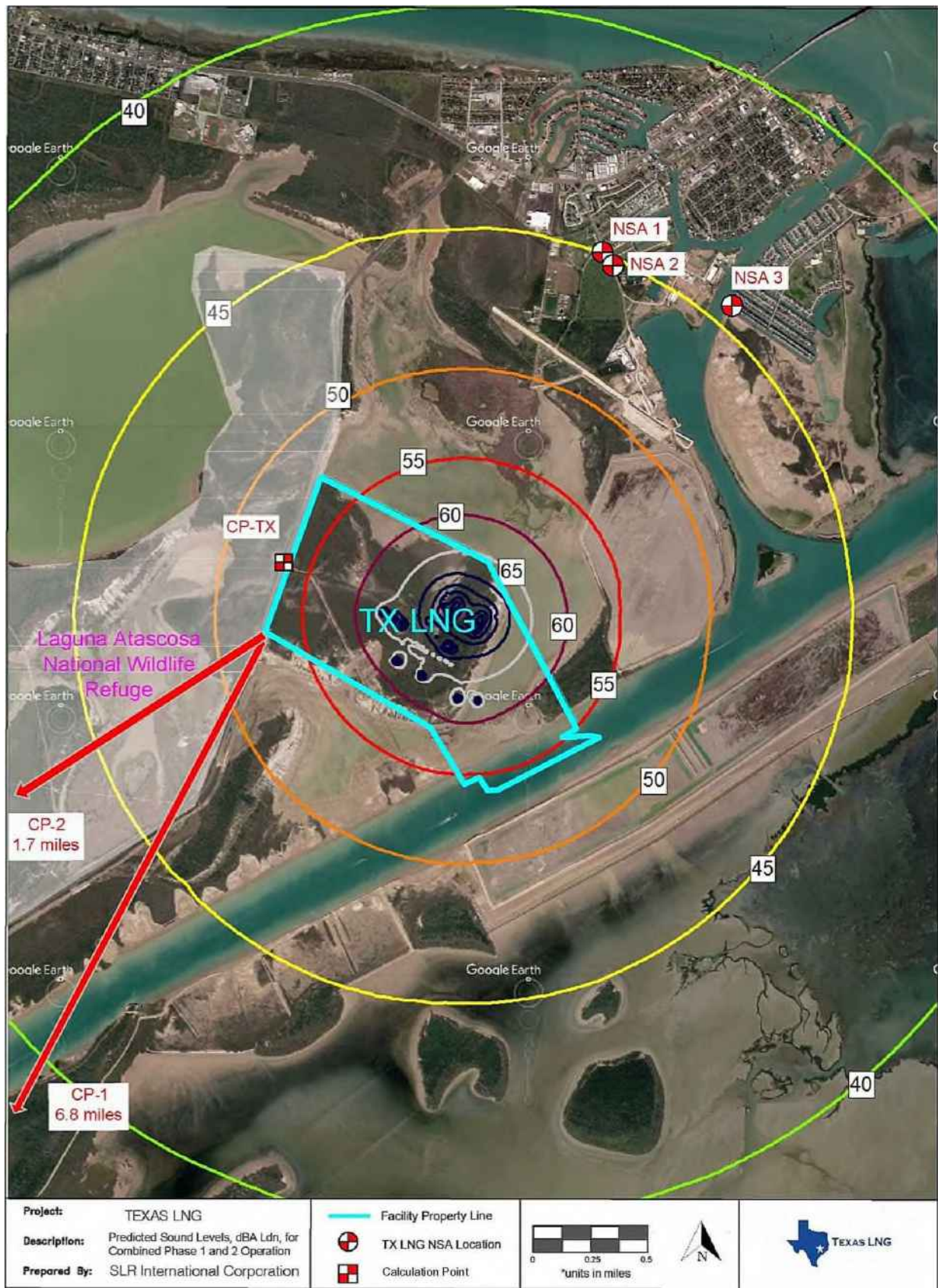
FIGURE 4.11.2-2 Predicted Sound Levels, dBA L dn , for Combined Phase 1 and 2 Operation
