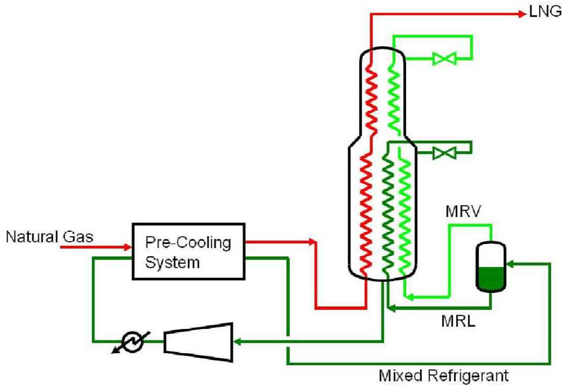
FIGURE 2.1.2-2 C3MR Process Schematic 15
