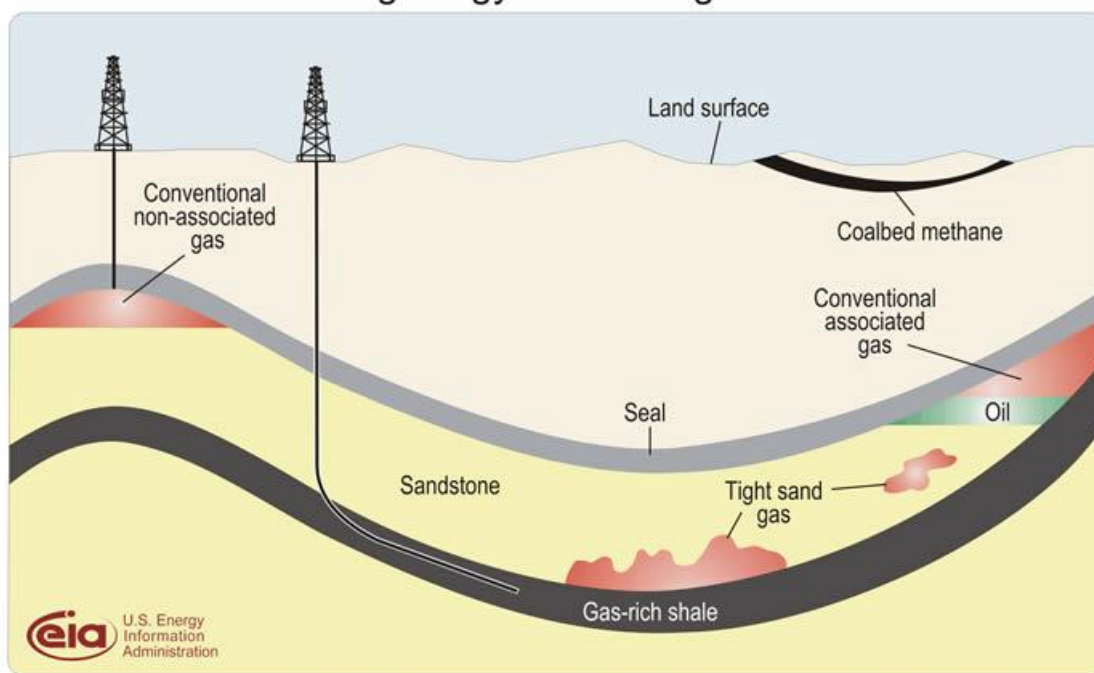
Figure 1. Geologic Nature of Major Sources of Natural Gas in the United States
