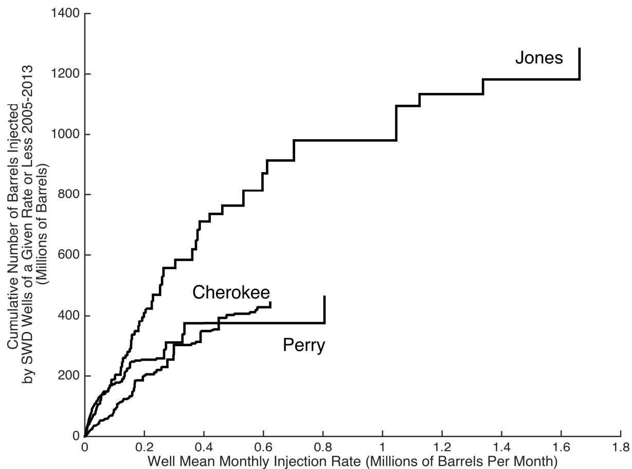
Fig. S2. Cumulative injection in the seismically active study areas as a function of the average injection rate of individual wells. 79% of the volume injected in the Cherokee area, 81% of the injected volume in the Perry area and 55% of the volume in Jones area was injected by wells injecting less than 400,000 barrels per month. Establishing an upper limit on disposal rates greater than this in each well may not significantly change injection patterns if a number of wells are used to inject the same aggregate volume in a given area.
