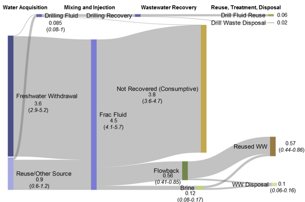
Figure 10. Sankey diagram of water volumes for the fracking water and wastewater management cycle estimated for this study, on a per well basis. “Frac” fluid dominates water use, and most is not recovered. Units = million gallons per well.
