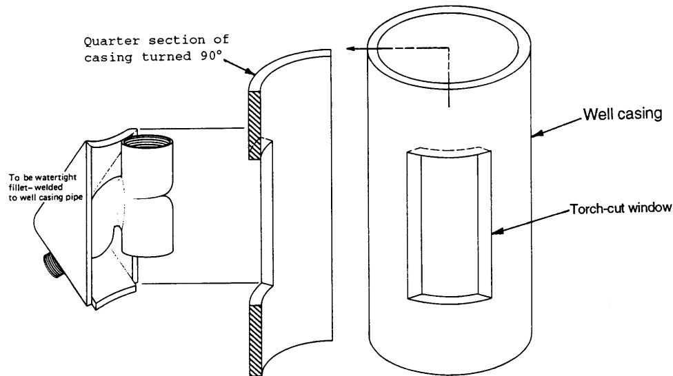
Figure 28. A weld-on pitless adapter.
