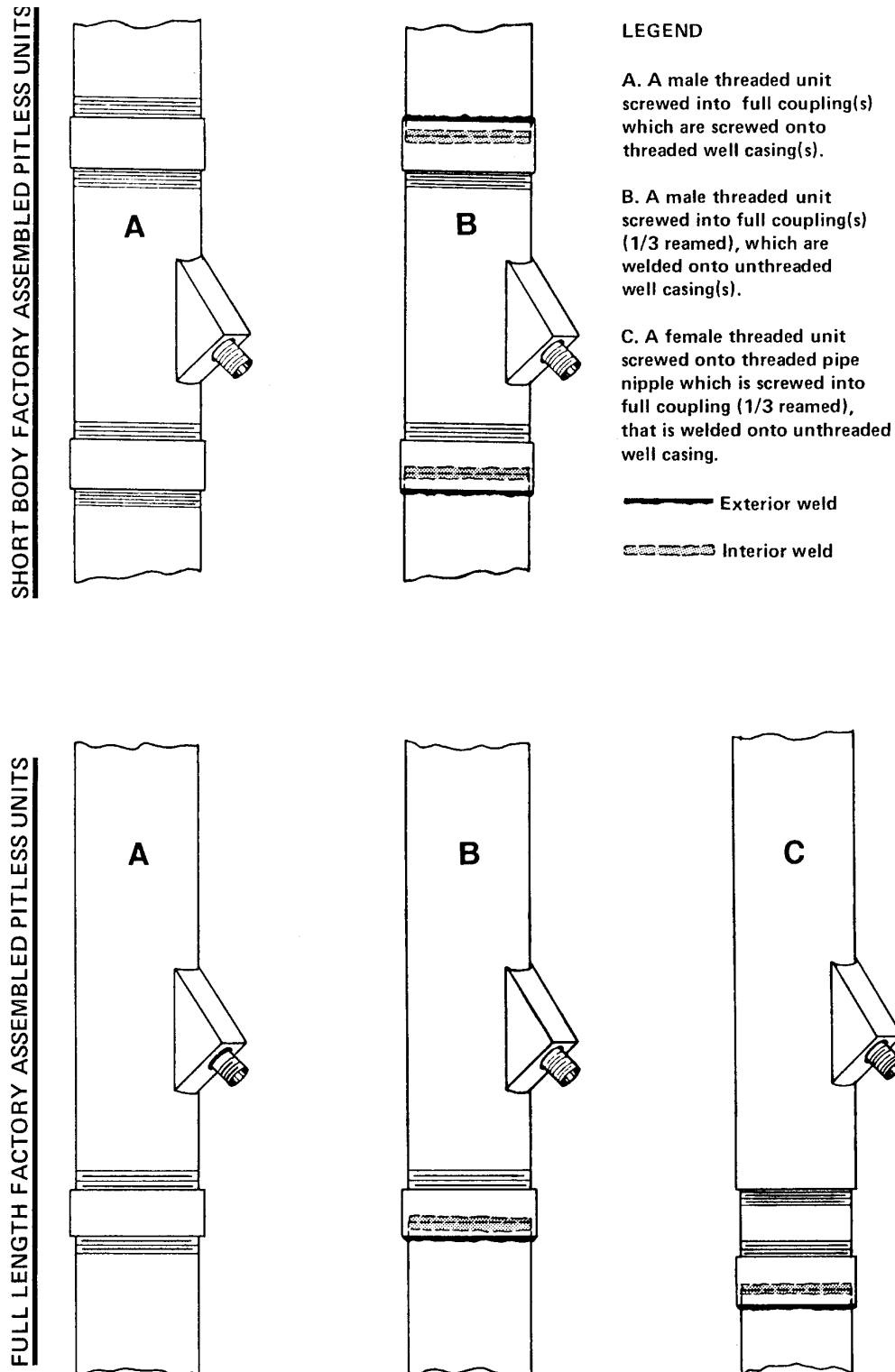
Figure 30. Pitless unit connections for wells with steel well casing pipe.
