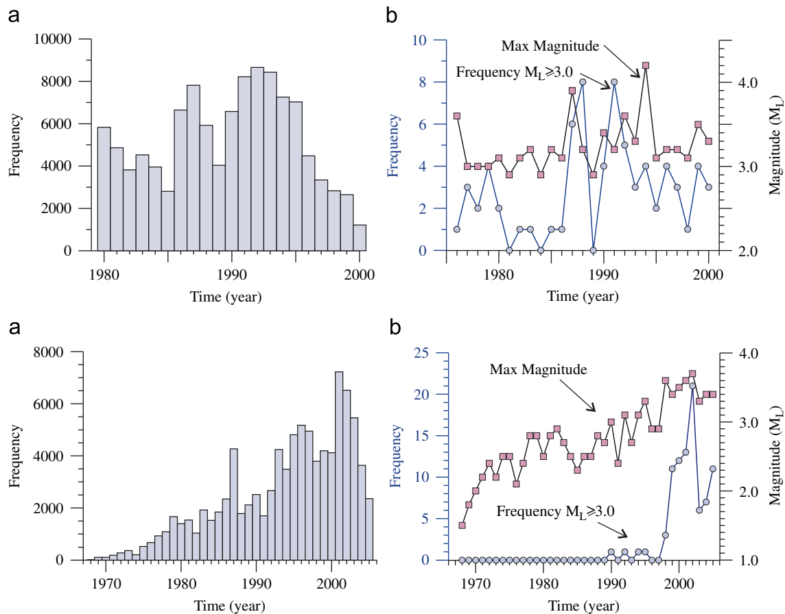
Fig. 21. Top panels: Mining-induced earthquakes at Mentougou coal mine, Beijing, (a) events M > 1.0 , (b) events M \geq 3.0 and the maximum event magnitudes. Bottom panels: same as top panels except for the Fushun coal mine field in Liaoning Province. (From Li et al. (2007)).
