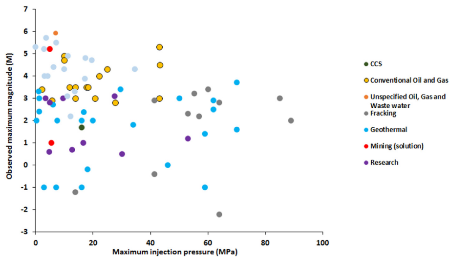
Fig. 98. M_{\text{MAX}} vs. maximum wellhead injection pressure for the 79 cases where data are reported.
