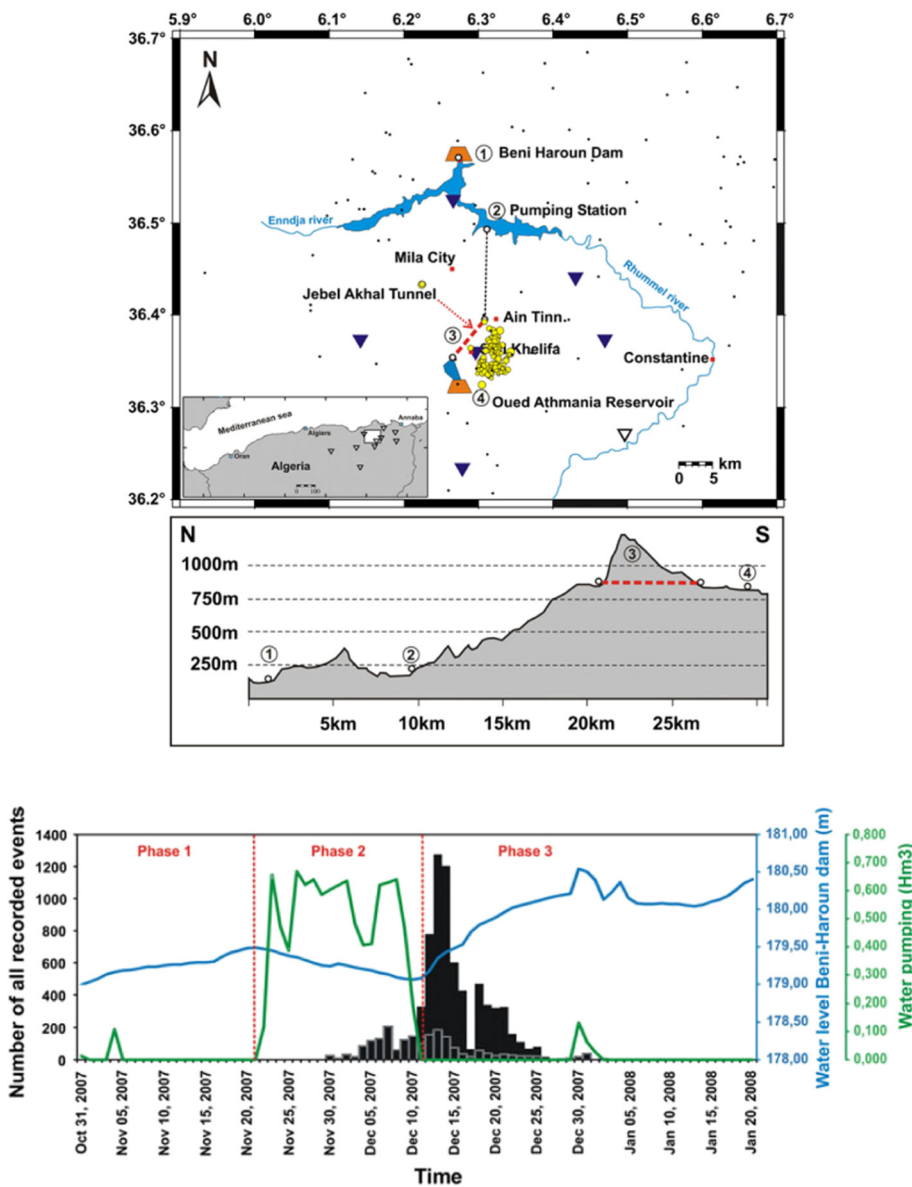
Fig. 10. Map of hydraulic system in Mila region, Algeria. Top: Water transport system (dashed lines) from Beni Haroun dam to Oued Athmania reservoir. Red dashed line: tunnel through Mt. Jebel Akhal; black dots: seismicity for 2006–2007; triangles: seismic stations; yellow dots: epicenters of earthquakes postulated to have been induced. Middle: topographic profile of hydraulic system. Bottom: Number of earthquakes recorded, water level in Beni Haroun dam, and volumes of water pumped vs. time around the seismogenic period. Black histogram: events recorded; gray histogram: events recorded by the network, discarding a temporary station deployed in the epicentral area for 17 days during the swarm. This exemplifies the effect of varying the number of seismic stations. (From Semmane et al. (2012).)
