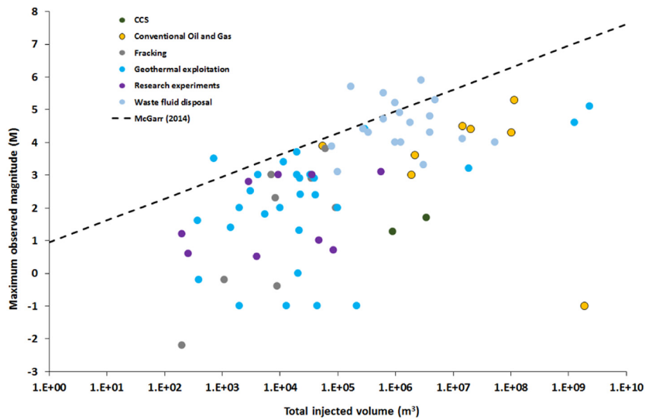
Fig. 97. M_{\text{MAX}} vs. total injected volume for the 69 cases of induced seismicity for which data are available. The upper-bound magnitude limit proposed by McGarr (2014) on the basis of theoretical considerations is also plotted.
