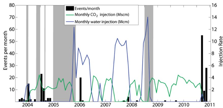
Fig. 79. CO 2 , water injection, and associated earthquakes at the Weyburn Oilfield, Saskatchewan, Canada. Shaded periods: monitoring array was inoperative. (From Verdon et al. (2013).)
