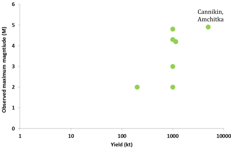
Fig. 101. M_{\text{MAX}} vs. yield in kilotonnes for nuclear tests that activated faults for the seven cases reported. Only one of these (Benham) is in common with the dataset of McKeown and Dickey (1969) .
