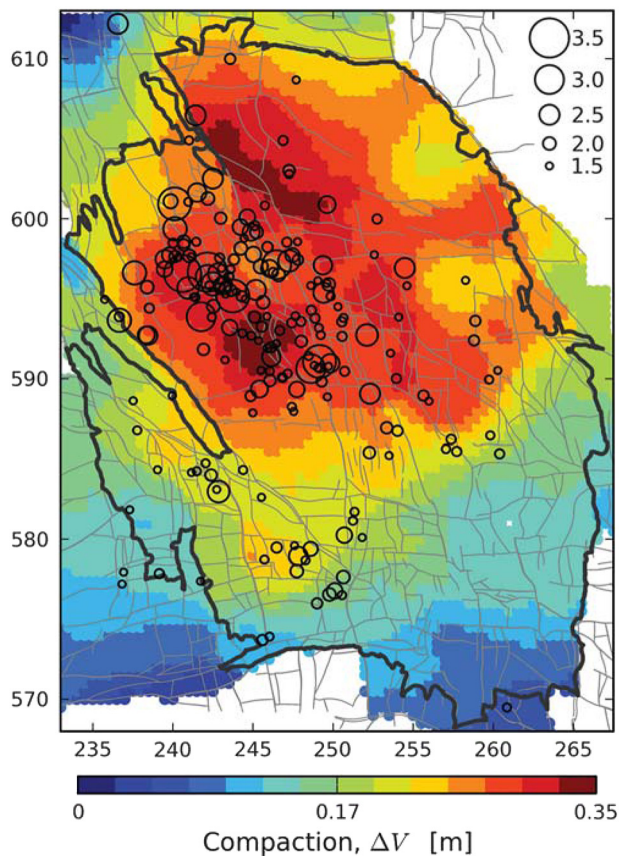
Fig. 35. The Groningen Gasfield. Earthquake epicenters for events with M \geq 1.5 for the period 1995–2012, superimposed on a model of reservoir compaction for 1960–2012. Black line: perimeter of the Groningen Gasfield; thin gray lines: faults close to the reservoir level. Map coordinates are kilometers in the Dutch national triangulation coordinate system (Rijksdriehoek). (From Bourne et al. (2015).)
