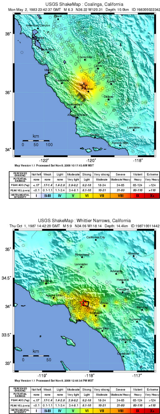
Fig. 39. U.S. Geological Survey shake maps ( http://earthquake.usgs.gov/earthquakes/shakemap/ ). Top: 1983 M_W 6.2 Coalinga, California earthquake, which injured 94 people and was felt throughout half the state. Bottom: 1987 M_L 5.9 Whittier Narrows, California earthquake, which killed six people. Ground shaking was felt throughout the regions shown in the maps and ranged from Light (cool colours) to Severe (warm colours). See the U.S. Geological Survey webpage for more details.
