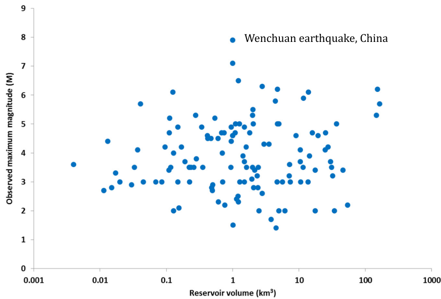
Fig. 91. Plot of M_{\text{MAX}} vs. water reservoir volume for the 126 cases for which data are available.
