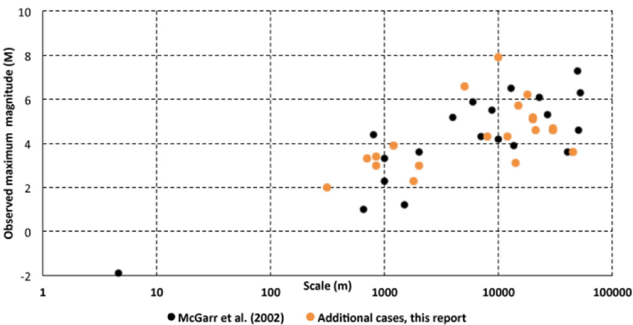
Fig. 102. M_{\text{MAX}} vs. project scale in meters. Black dots: cases studied by McGarr et al. (2002) ; orange dots: 20 additional cases from our database. Project scale was estimated using the longest dimension of the project, e.g., the length of a water reservoir.
