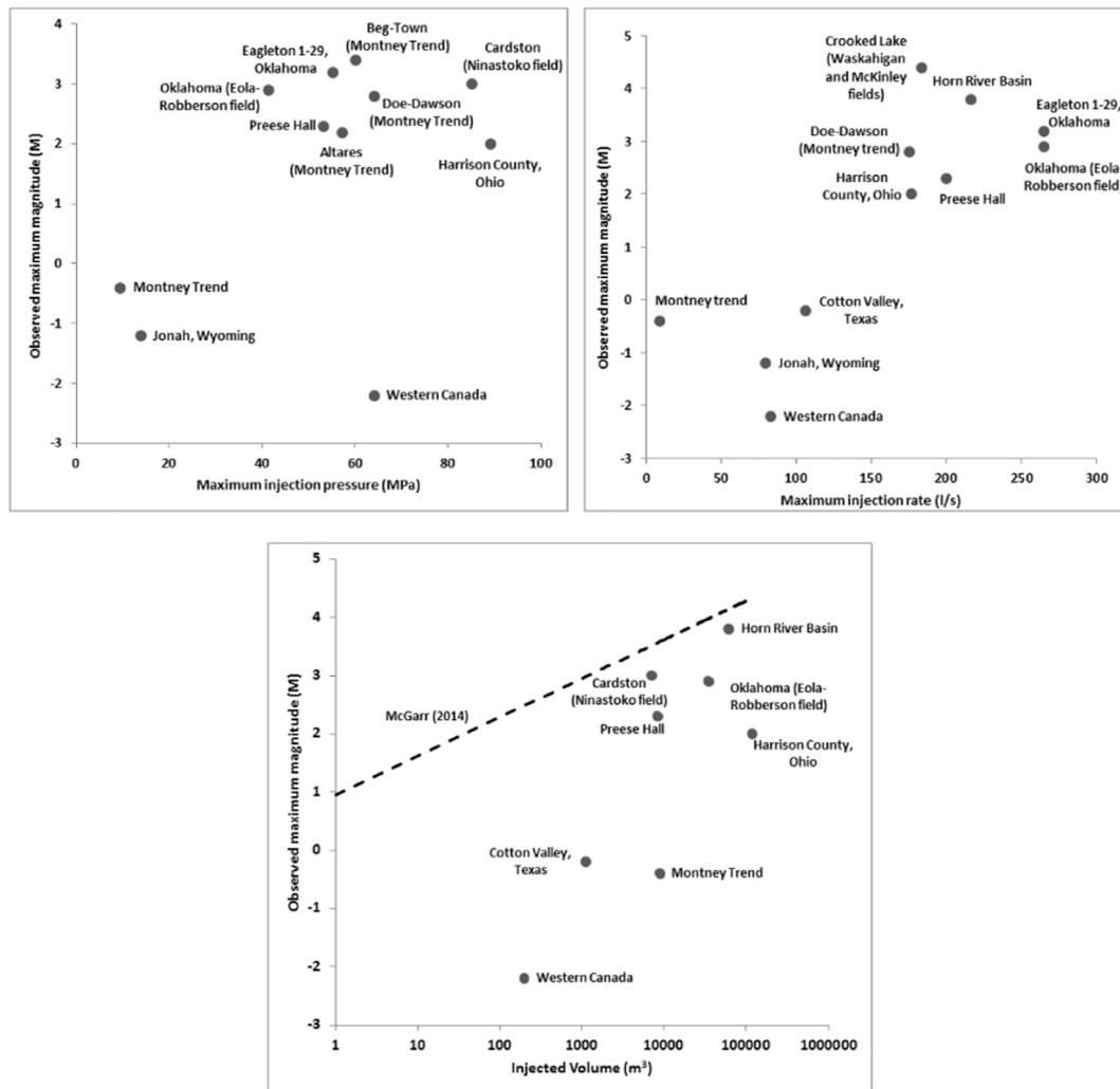
Fig. 96. For all cases of shale-gas hydrofracturing-induced earthquakes in our database where data are available, top left: M_{\text{MAX}} vs. maximum injection pressure, top right: M_{\text{MAX}} vs. maximum injection rate, and bottom: M_{\text{MAX}} vs. injected volume.
