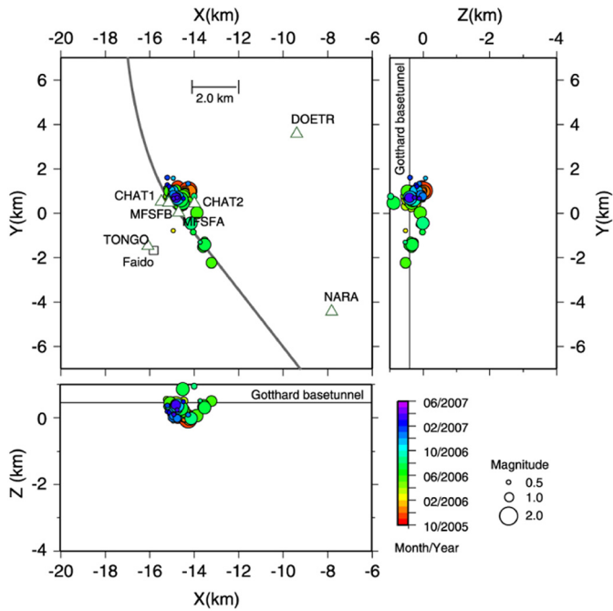
Fig. 27. Hypocenter locations of earthquakes in the vicinity of the multi-function station Faïdo, Switzerland, October 2005–June 2007. (From Husen et al. (2012).)
