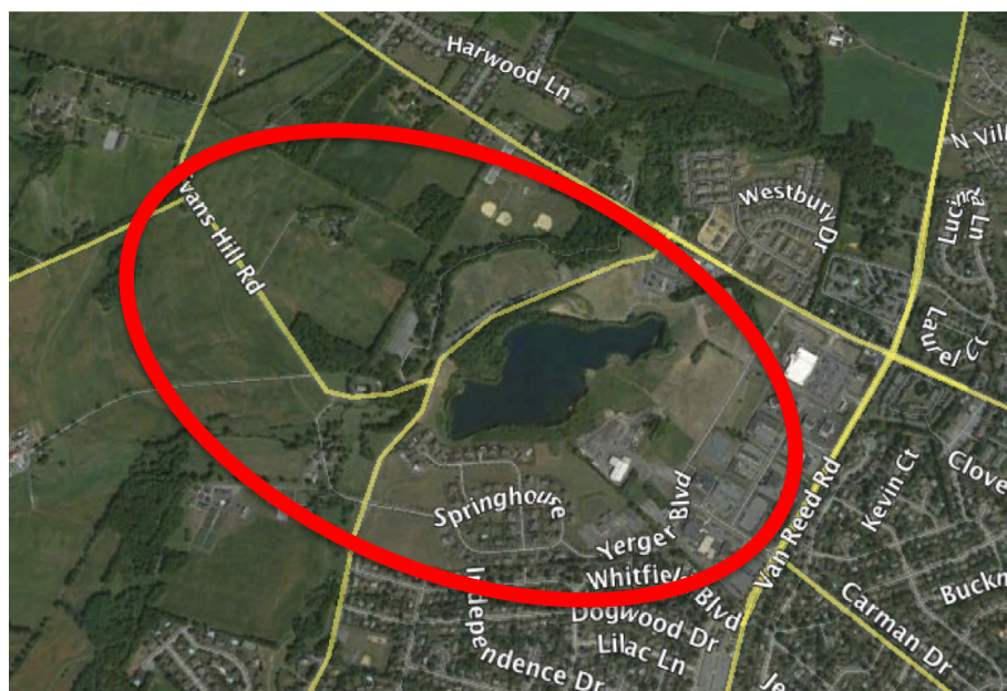
Fig. 69. Site of the former Cacoosing Valley, Pennsylvania, quarry. Red oval: approximate boundary of the old quarry. Satellite image from Google Maps.
