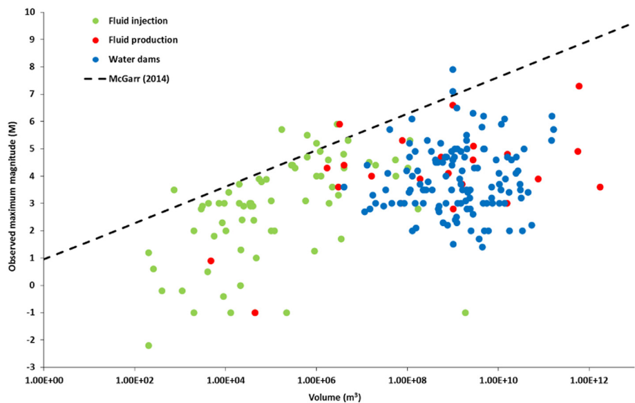
Fig. 99. M_{\text{MAX}} vs. volume or proxy volume of material removed or added for the 218 cases for which data are available, along with the relationship proposed by McGarr (2014) on the basis of theoretical considerations. Volumes and proxy volumes were estimated as follows: Water dams—the volume of the impounded reservoir; fluid injection or extraction—fluid volume injected into or extracted from the subsurface; mining—mass of material excavated, converted to volume using an appropriate density; construction—relevant mass converted to volume using an appropriate density for the building materials; CCS—mass of injected \text{CO}_2 converted to volume using a density of liquid \text{CO}_2 of 1100 \text{ kg/m}^3 .
