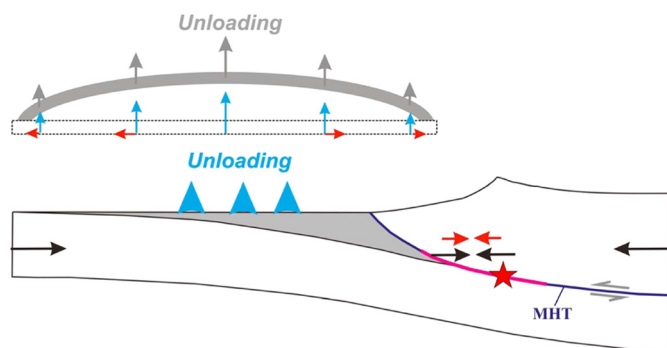
Fig. 18. Schematic diagram showing the effect of unloading by anthropogenic ground-water loss on the Main Himalayan Thrust. Dewatering induces a component of horizontal compression (red arrows) that adds to the secular interseismic contraction (black arrows) at seismogenic depths. Red star: the 2015 Gorkha, Nepal earthquake; pink line: the associated rupture.
