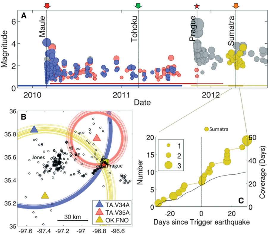
Fig. 58. Earthquakes in the Prague, Oklahoma, area. (A) Detected events, showing triggering by the 2010 Maule, Chile earthquake. Red star: the 6 November 2011 Mw 5.7 Prague earthquake. (B) Distances to detected events. (C) Cumulative number of events in the time period surrounding the 11 April 2012 Mw 8.6 and 8.2 Sumatra earthquakes. (From van der Elst et al. (2013).)
