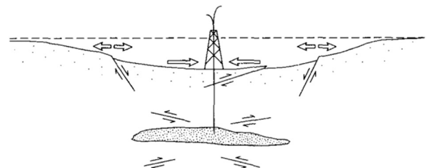
Fig. 38. Schematic cross section summarizing surface deformation and faulting associated with fluid withdrawal. Normal faults develop on the flanks of the field, as observed at the Goose Creek, Texas, Oilfield. Reverse faults develop above reservoirs as observed at Wilmington, Buena Vista Hills, the Pau Basin and beneath the Strachan Field. (From Segall (1989).)
