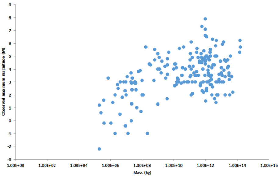
Fig. 100. M_{\text{MAX}} vs. mass of material removed or added for the 203 cases where data are available. Water volumes were converted to mass using a density 1000 \text{ kg/m}^3 . Oil and gas are not included in this plot except where quantity was reported in units of mass. Project types plotted include CCS, construction, conventional oil and gas, shale-gas hydrofracturing, geothermal, mining, research experiments, waste fluid injection and water reservoirs.
