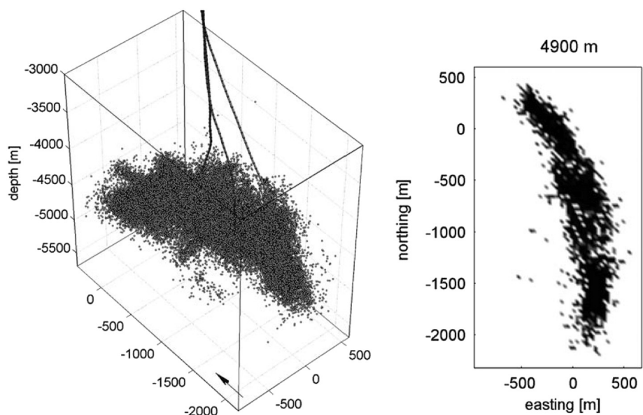
Fig. 60. Top left: Distribution of earthquake hypocenters at the Soultz-sous-Forêts EGS project in perspective view. Solid lines: wells GPK2, GPK3 and GPK4. Top right: Depth slice of the hypocenter density distribution at 4900 m depth. Dark shading: regions of high density. (From Baisch et al. (2010).)
