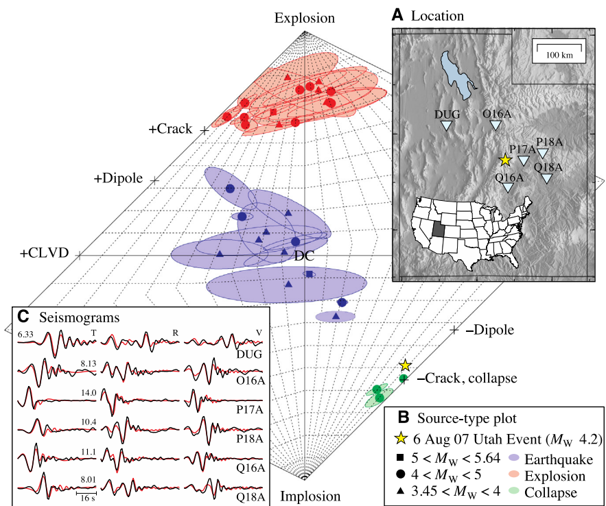
Fig. 22. (A) Locations of the 6 August 2007 Crandall mine, Utah, earthquake and six of the closest USArray and Advanced National Seismic System (ANSS) seismic stations. (B) Source-type plot showing separation of populations of earthquakes, explosions, and collapses. Yellow star shows the focal mechanism solution. (C) Observed seismograms (black) compared to synthetics (red) for the solution, which is similar to a horizontal closing crack (B). The maximum displacement (10–7 m) of each set of tangential (T), radial (R), and vertical (V) observations is given. (From Dreger et al. (2008).)
