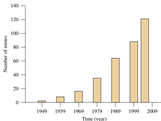
Fig. 20. Number of mines in China with rockburst hazard vs. time.
